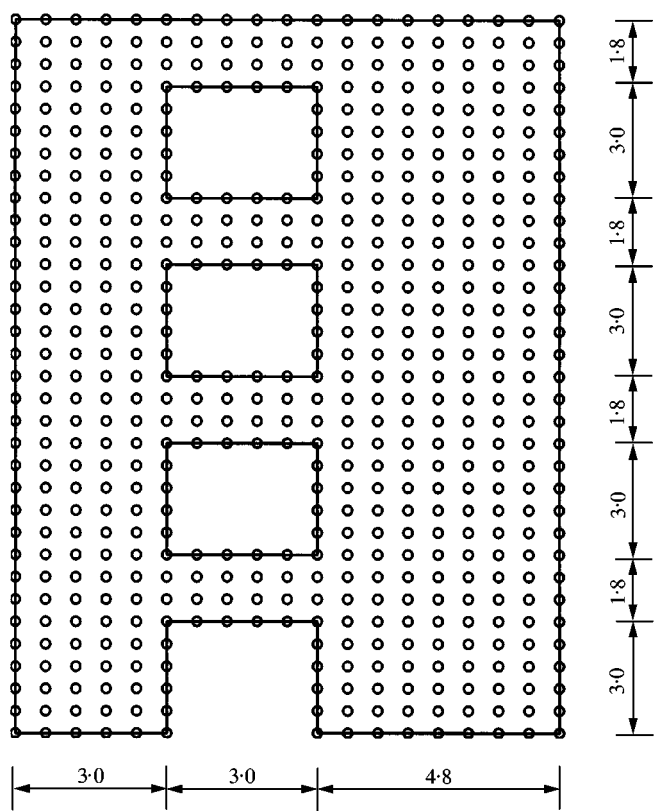
Figure 10. A shear wall with four openings.
